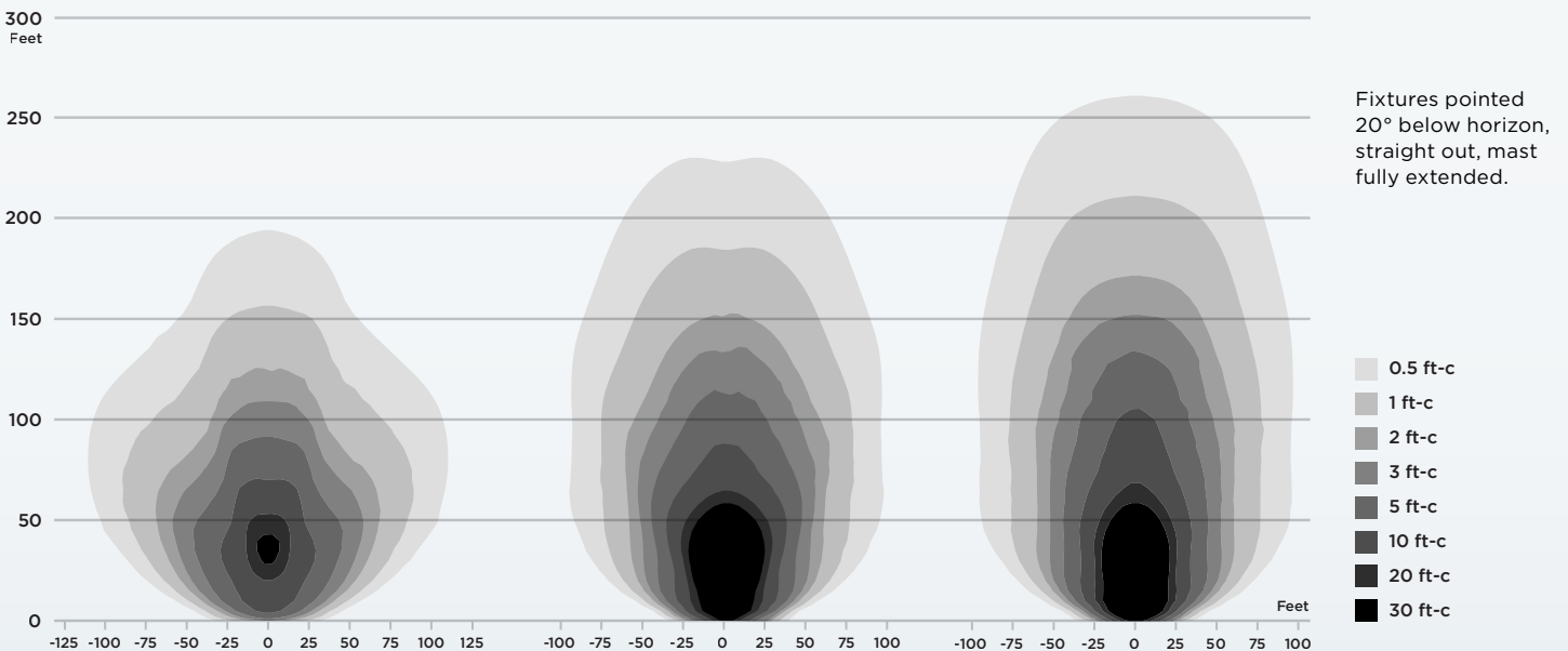
Night-Lite Pro II® V-Series® with four 320-W LED Light Output
